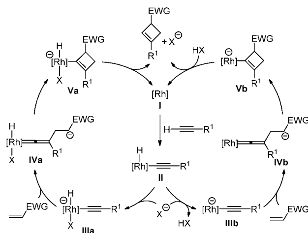
Figure 1. Proposed mechanisms of the [2 + 2] cycloaddition.
